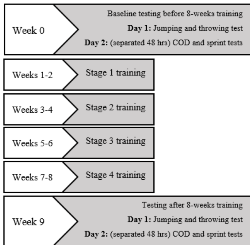
Figure 1. Testing timeline; COD: change of direction.
